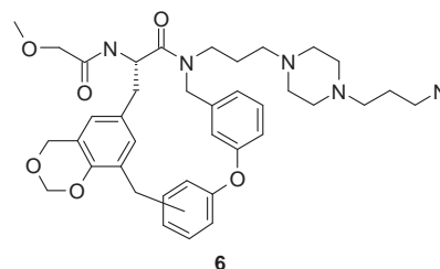
Scheme 5. Proposed structure 6 .
