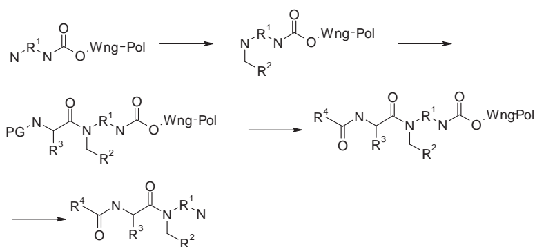
Scheme 2. Outline of the synthesis.
