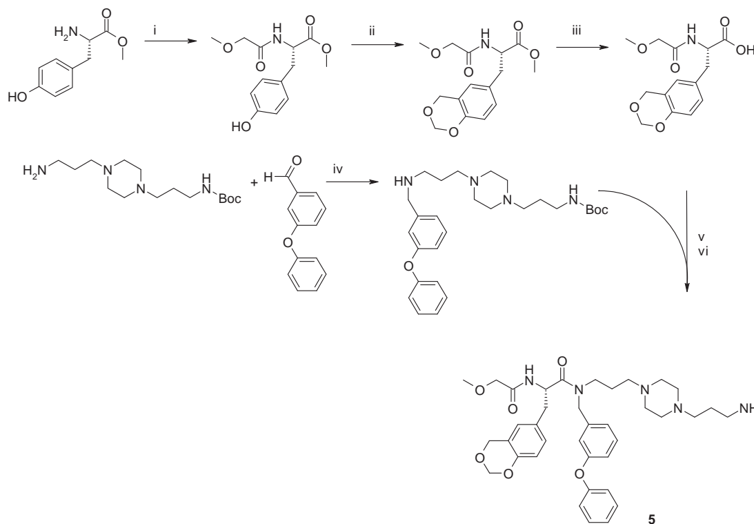
Scheme 4. Synthesis of compound 5 . Reagents and conditions: (i) 1 equiv HOBT, 1 equiv TBTU, 1.5 equiv DIPEA; (ii) TFA/DCM 1:1, 2 equiv paraformaldehyde, 1 h; (iii) LiOH, H 2 O. (iv) ethanol, Raney-Ni, H 2 ; (v) 1.2 equiv 2,4,6-tripropyl-1,3,5,2,4,6-trioxatriphosphorinane-2,4,6-trioxide (PPAA), 5.9 equiv N -methyl morpholin, DCM; (vi) TFA.
