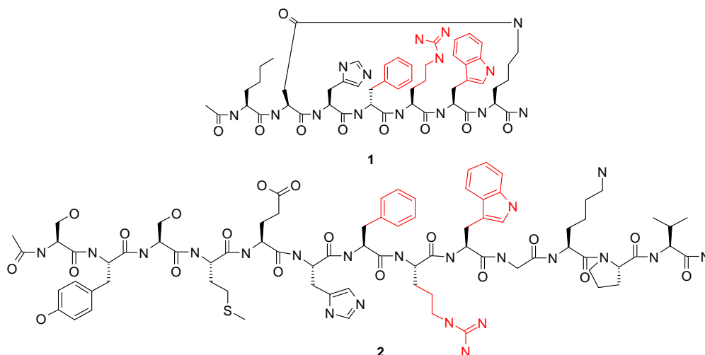
Scheme 1. MT-II (1) and \alpha -MSH (2). The important pharmacophores are shown in red.
