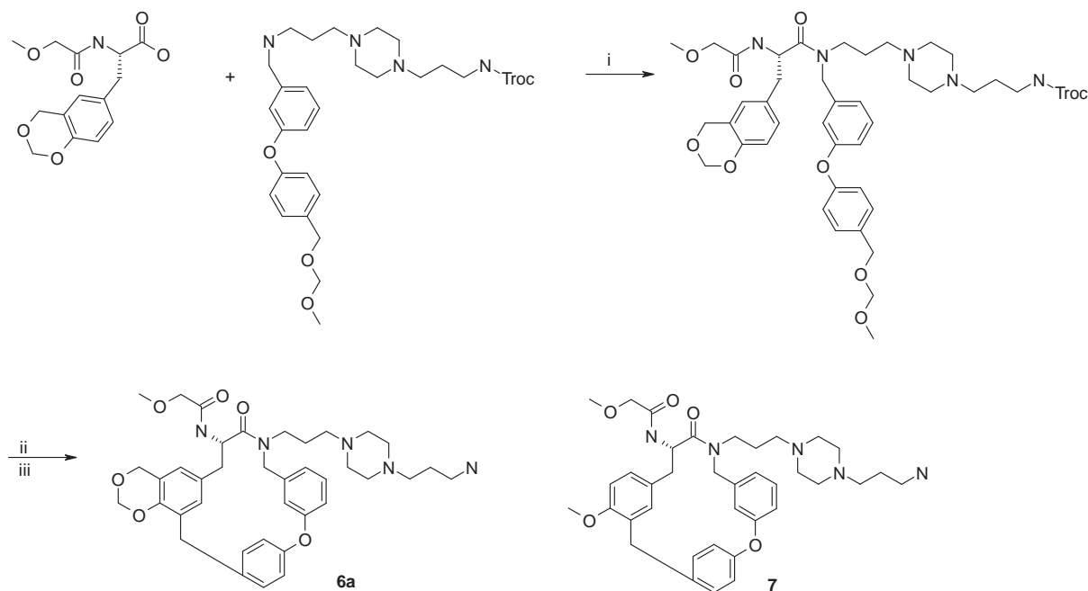
Scheme 6. Synthesis of macrocycle 6a and structure of macrocycle 7 . Reagents and conditions: (i) 1.5 equiv collidine, 1.5 equiv HATU, DCM; (ii) TFA/DCM 1:1 90 min; (iii) Zn, HOAc.
