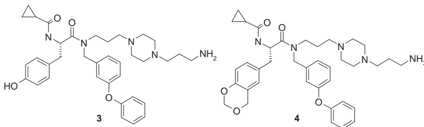
Scheme 3. Intended structure 3 and 4 H -benzo[1,3]dioxin 4 .
